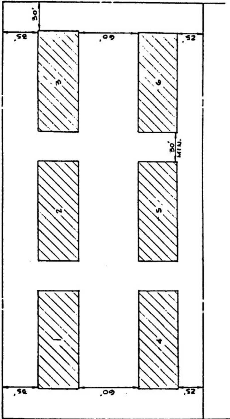
FIG. I APARTMENT OR TOWNHOUSE MINIMUM REQUIREMENTS (12 UNITS MAXIMUM PER BLDG.)
