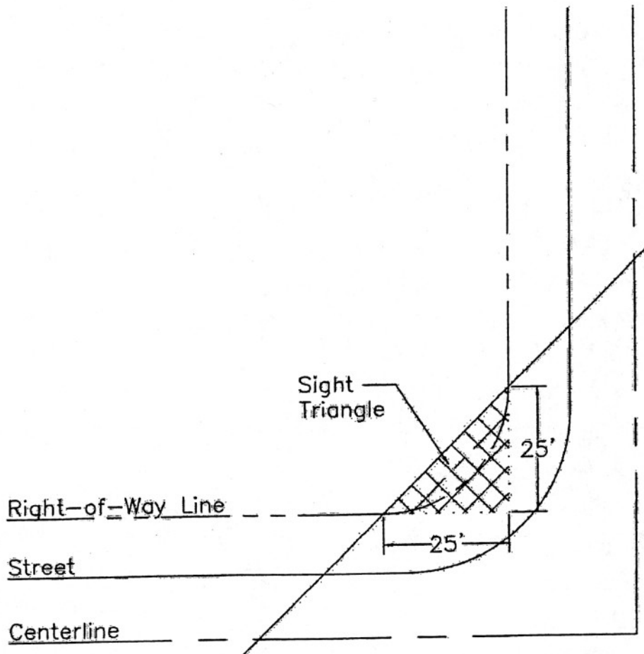
FIGURE 2 Standard Sight Triangle
