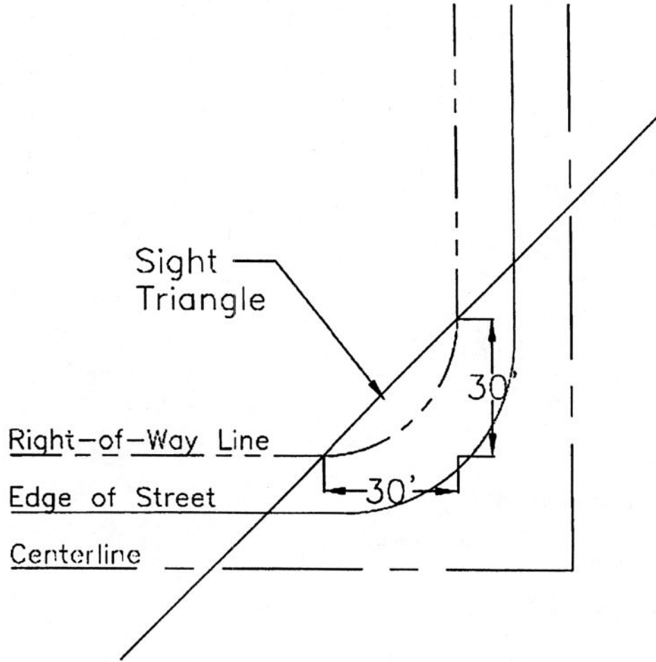
FIGURE 2 Standard Sight Triangle [Ord. No. 1140 §6, 3-21-2007]
