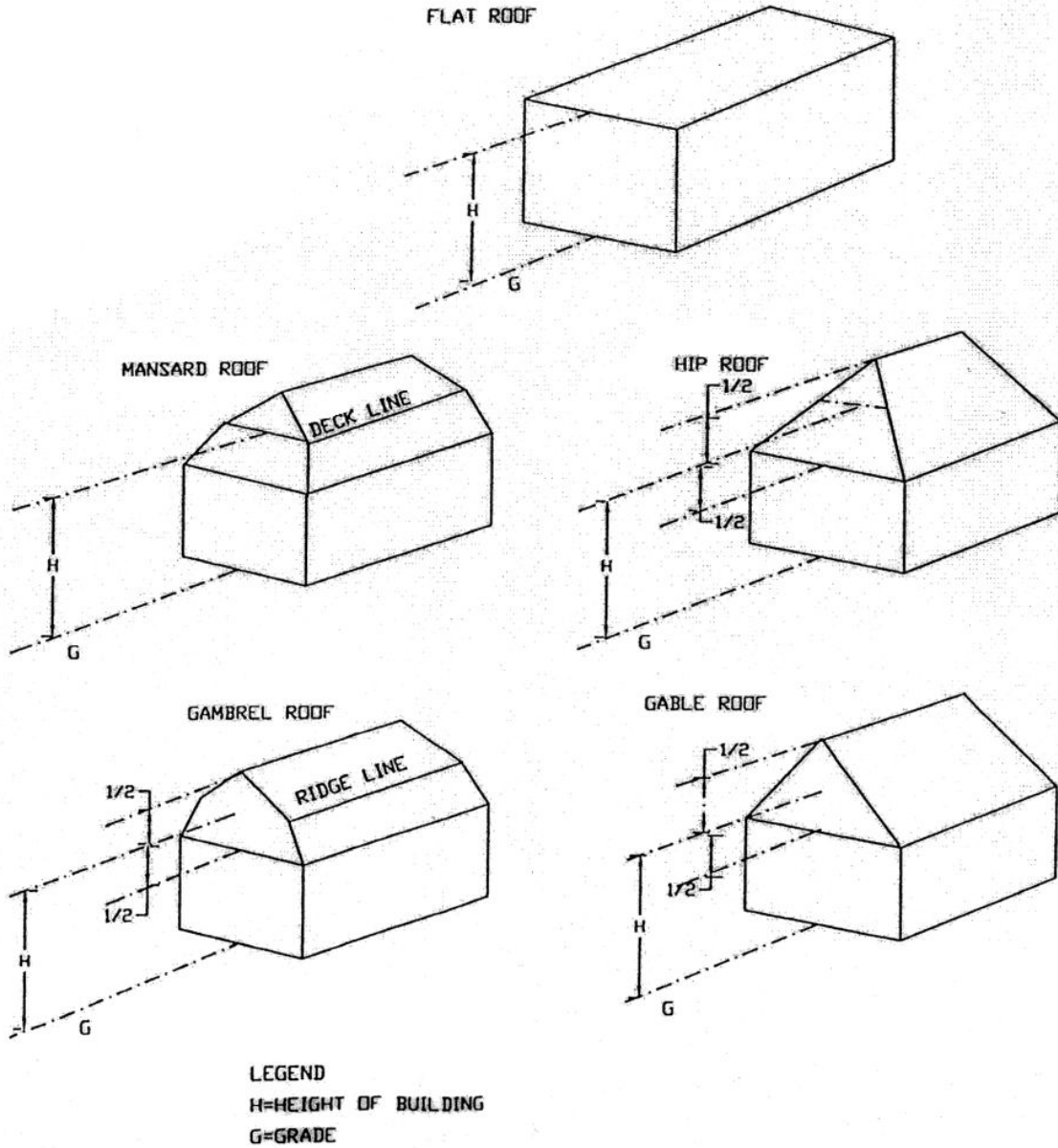
FIGURE 1 Illustration of Roof Line
