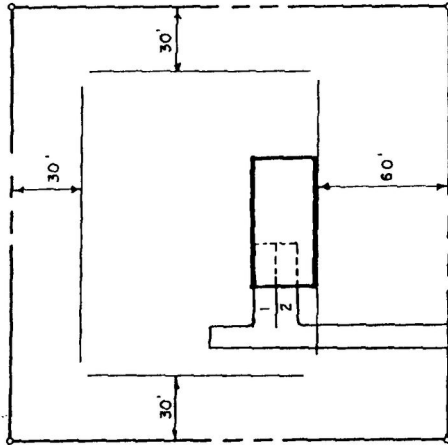
B) Example: 2 required parking spaces for single family dwelling with 2 car garage.
