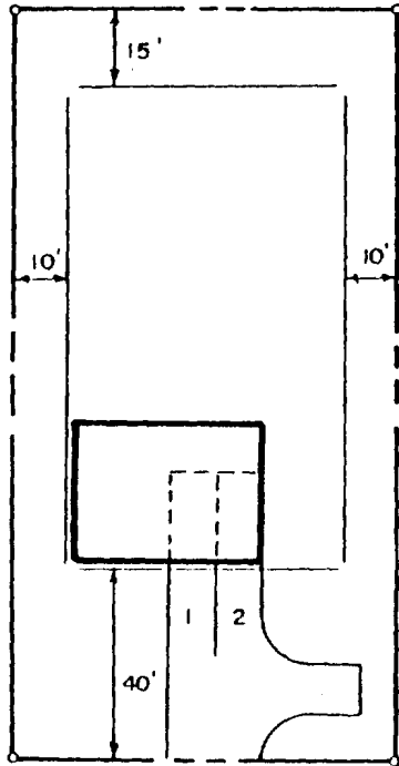
A) Example: 2 required parking spaces for single family dwelling with 2 car garage and double drive- way.
