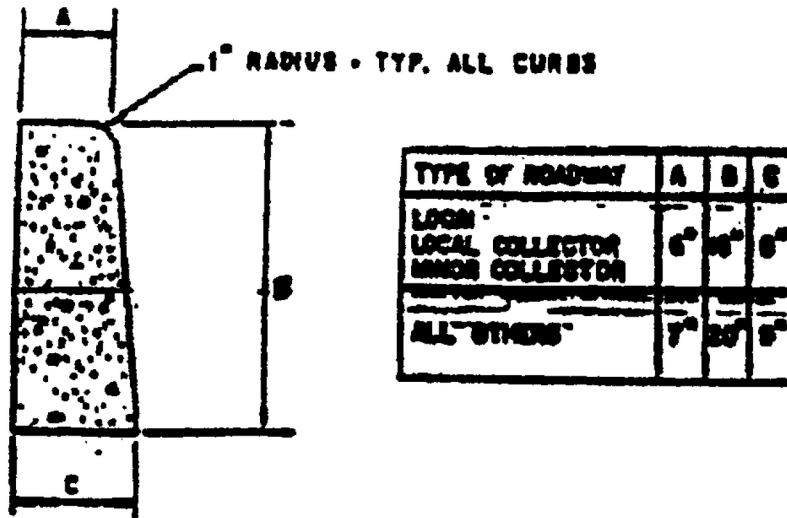
Figure 3 Concrete Curb
