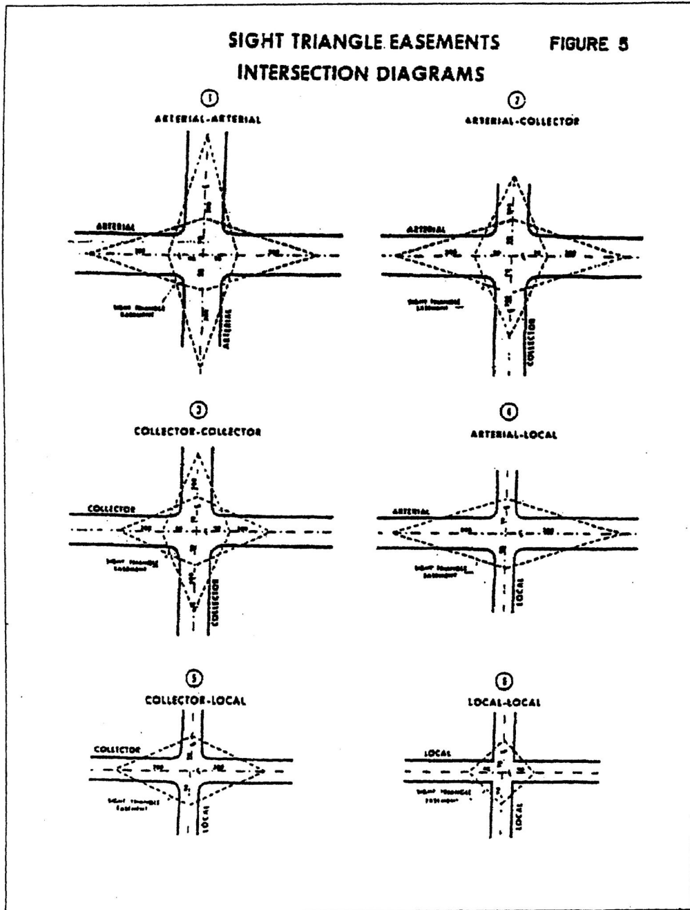
Figure 5 Sight Triangle Easements Intersection Diagrams
