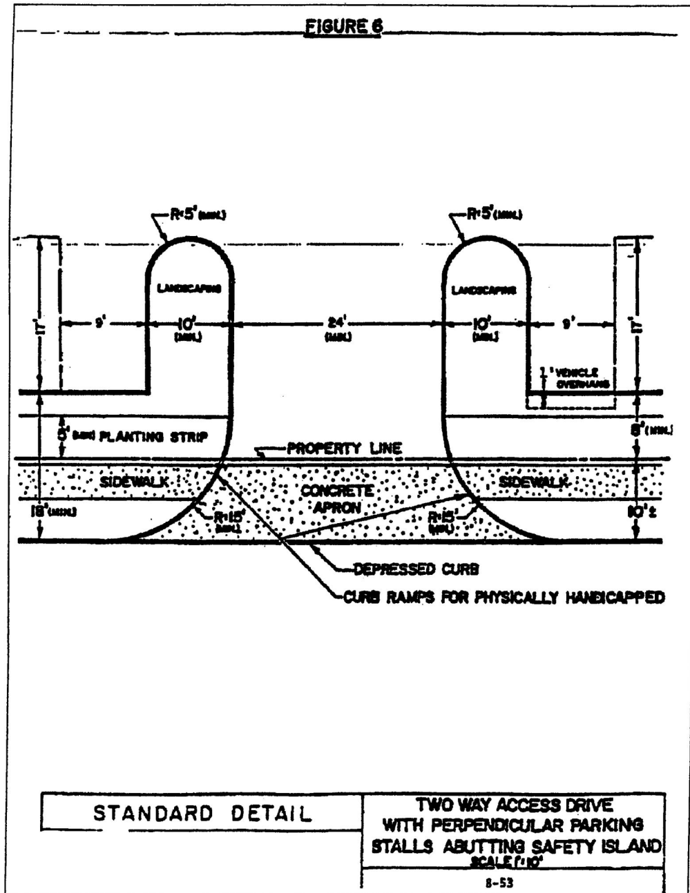
Figure 6 Two-Way Access Drive with Perpendicular Parking Stalls Abutting Safety Island
