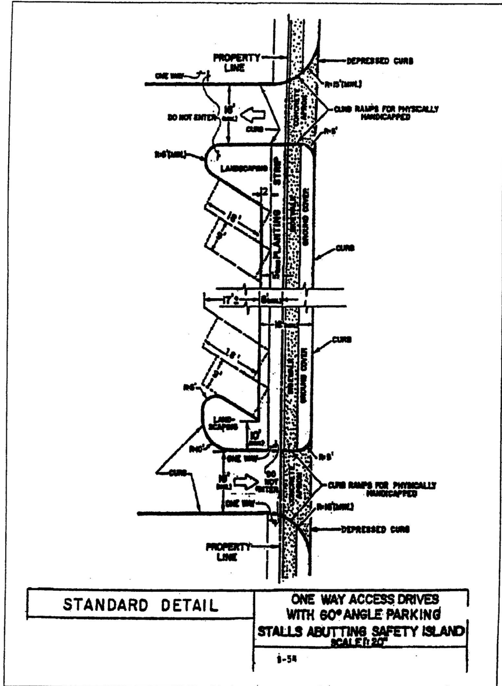
Figure 7 One-Way Access Drive with 60° Angle Parking Stalls Abutting Safety Island
