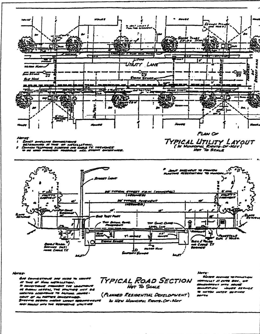
Figure 10 Typical Road Section
