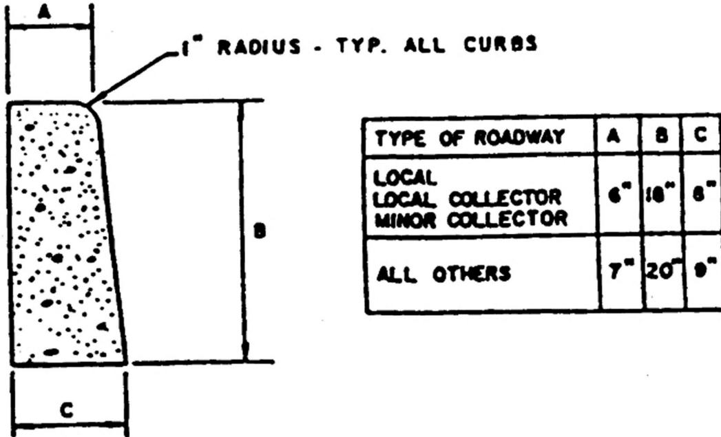
FIGURE VIII-3 CONCRETE CURB NOT TO SCALE
