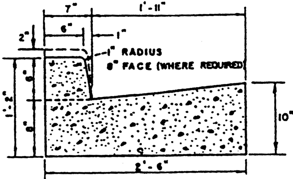
FIGURE VIII-4 COMBINATION CURB & GUTTER NOT TO SCALE
