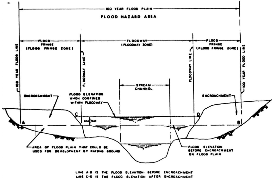
FLOOD PLAIN DIAGRAM
