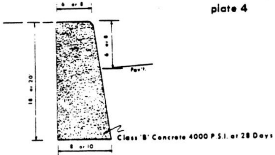
CURB DETAIL
