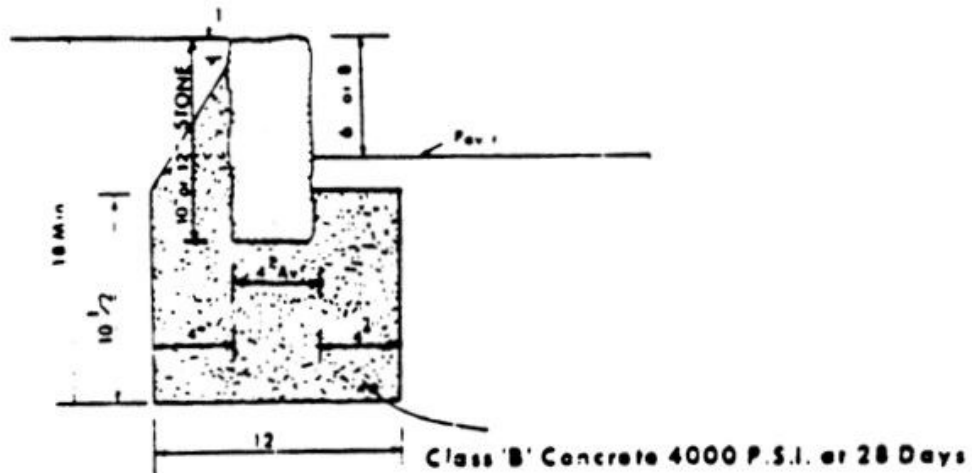
GRANITE or BELGIAN BLOCK CURB DETAIL
