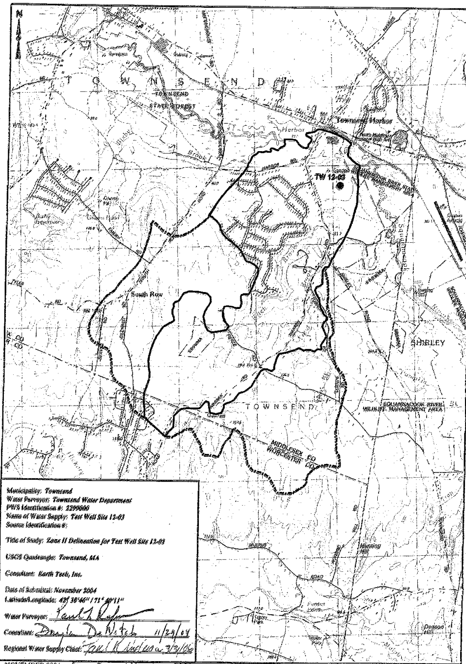
FIGURE 5-2 ZONE II AND ZONE III Harbor Trace Well Townsend Massachusetts November 29, 2004 DEP Endorsed 3/31/06
