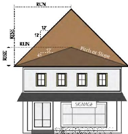
B. Example of roof treatment (b) if sloped, roof pitch shall be between 4/12 and 12/12
