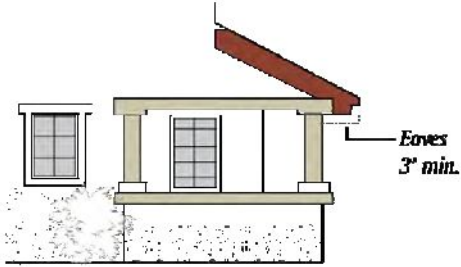
A. Example of roof treatment (a) Graphic reflects overhanging eaves as applied to gable, hip, and gambrel roofs
