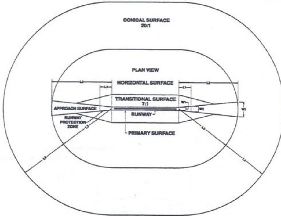
FAR Part 77 “Imaginary Surfaces” Dimension 1 Requirements
