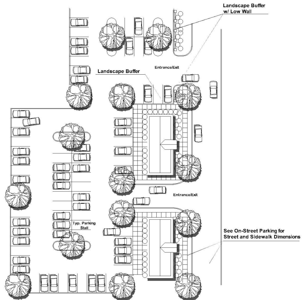
Figure 2 Surface Parking Designs
