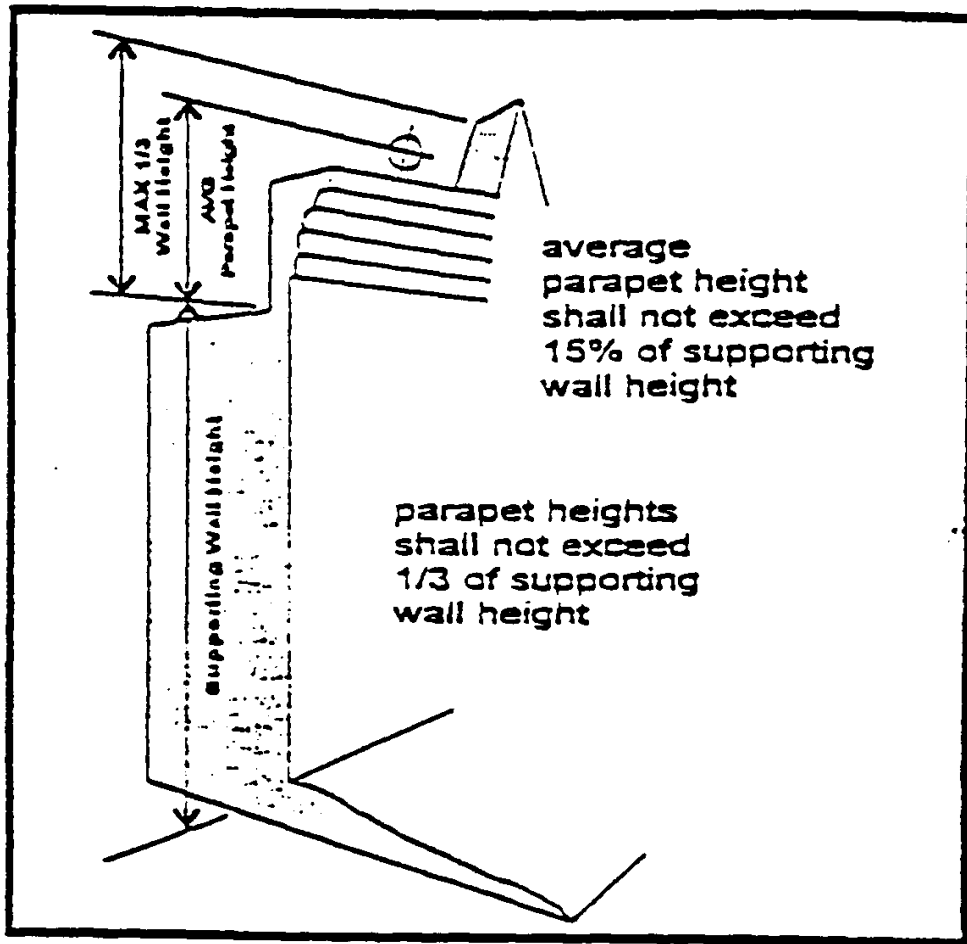
Parapet Standards.
