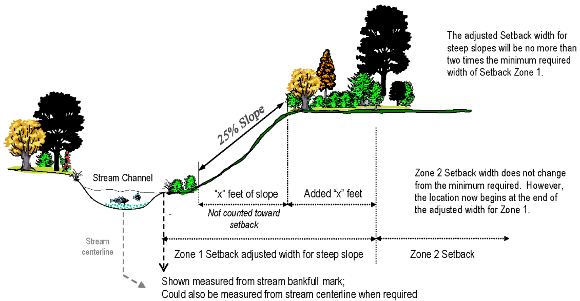
Figure 4 – Stream Setback adjustment for 25% slope or greater
