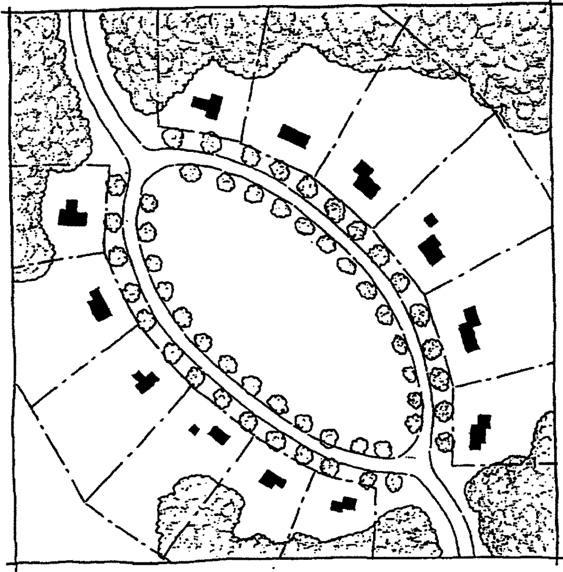
Figure 603-E(2) An example neighborhood cluster oriented toward common green and streetscape
