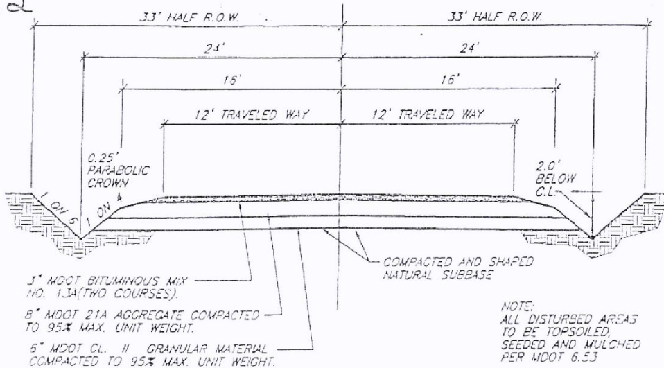
TYPICAL PAVED ROAD SECTION
