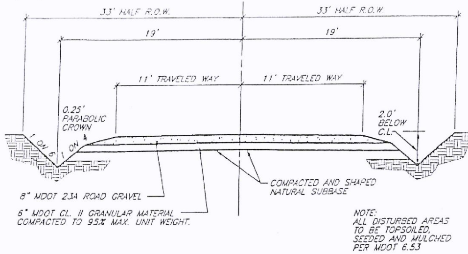
TYPICAL GRAVEL ROAD SECTION
