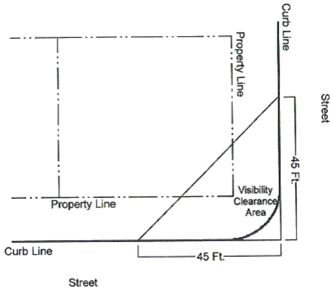
FIGURE 6 VISIBILITY CLEARANCE AREA
