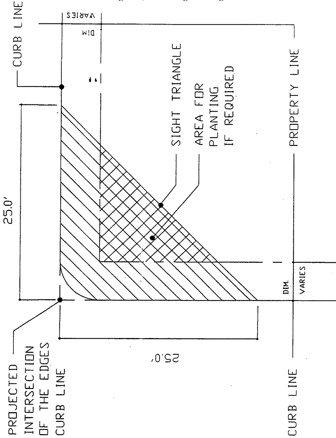
Figure 1, Corner Sight Triangle
