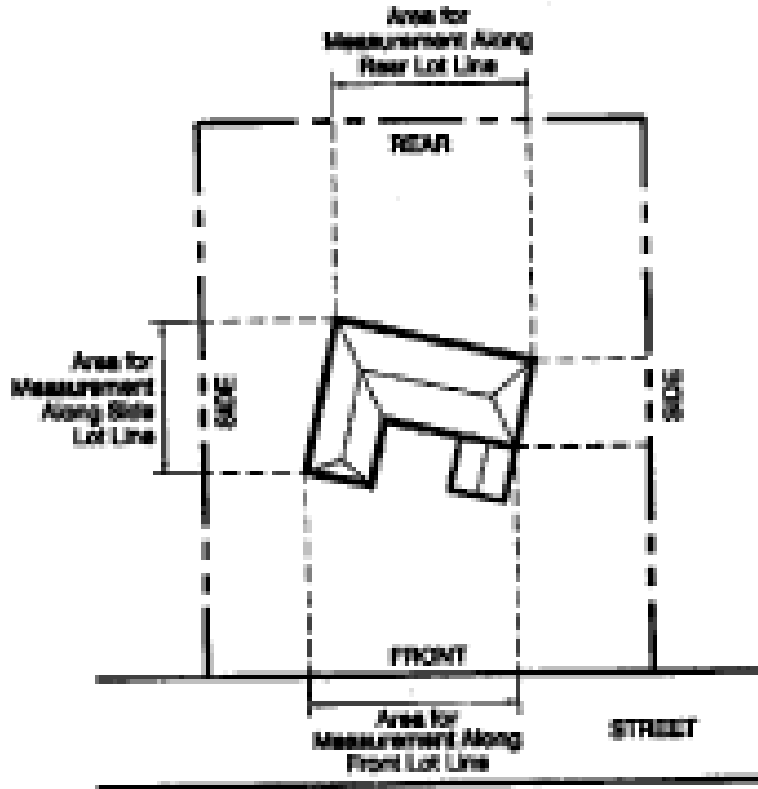
Figure 2-11.1: Area for Measurement Along Lot Lines
