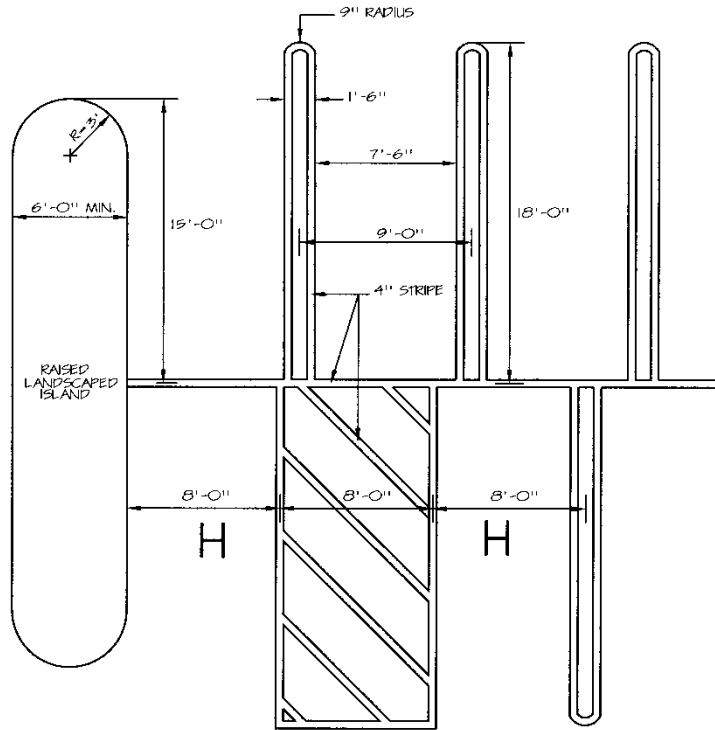
Figure 7-1: Typical Parking Space Details
