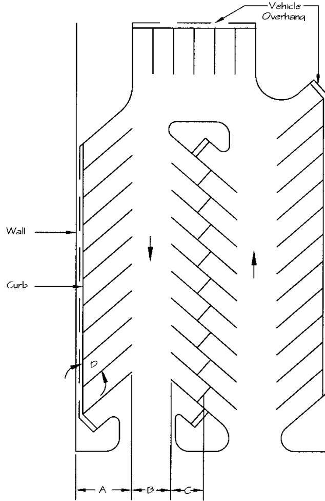
Figure 7-3: Sample Parking Layout-Angled Parking
