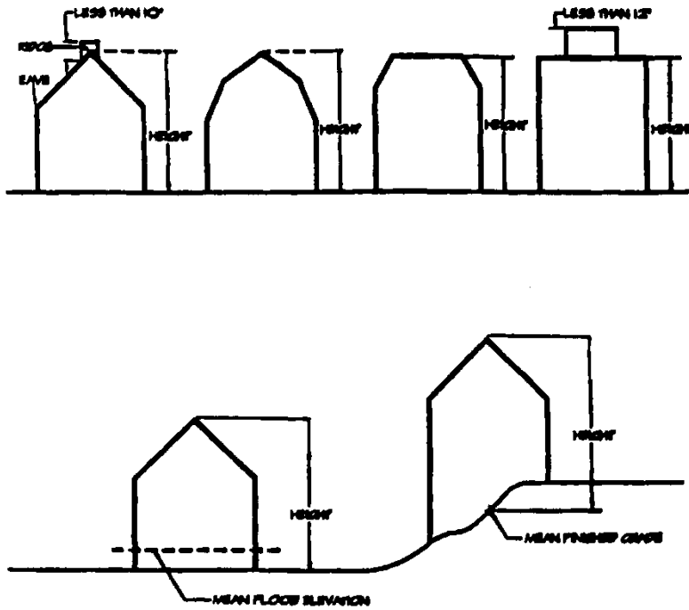
Figure 2-4: Measuring Height of a Building [Amended 7-22-2003 by L.L. No. 7-2003; 10-16-2012 by L.L. No. 3-2012]
