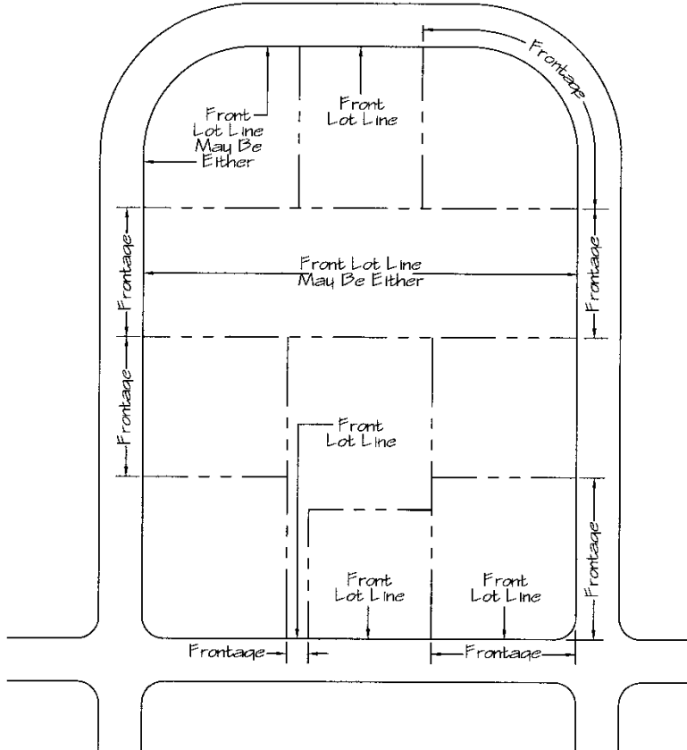
Figure 2-6: Front Lot Line and Frontage
