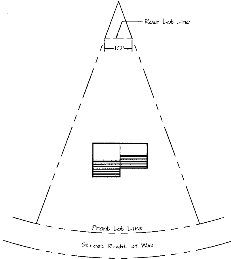
Figure 2-7: Rear Lot Line
