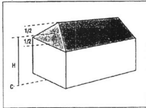
Gable Roof
