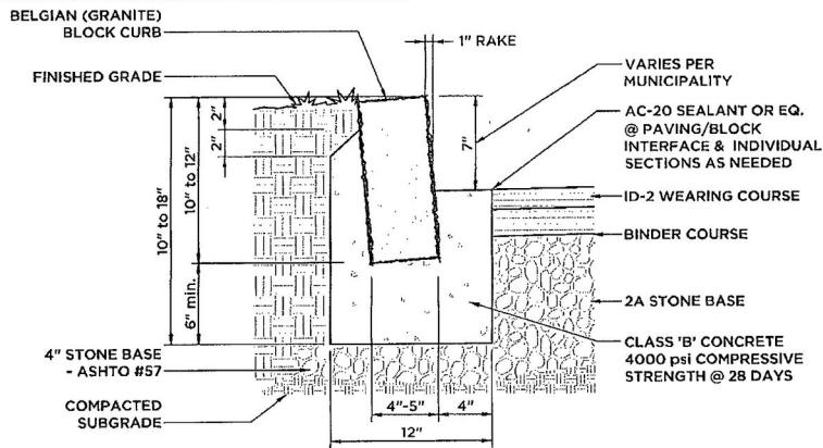
○ GRANITE BLOCK CURB DTL.
