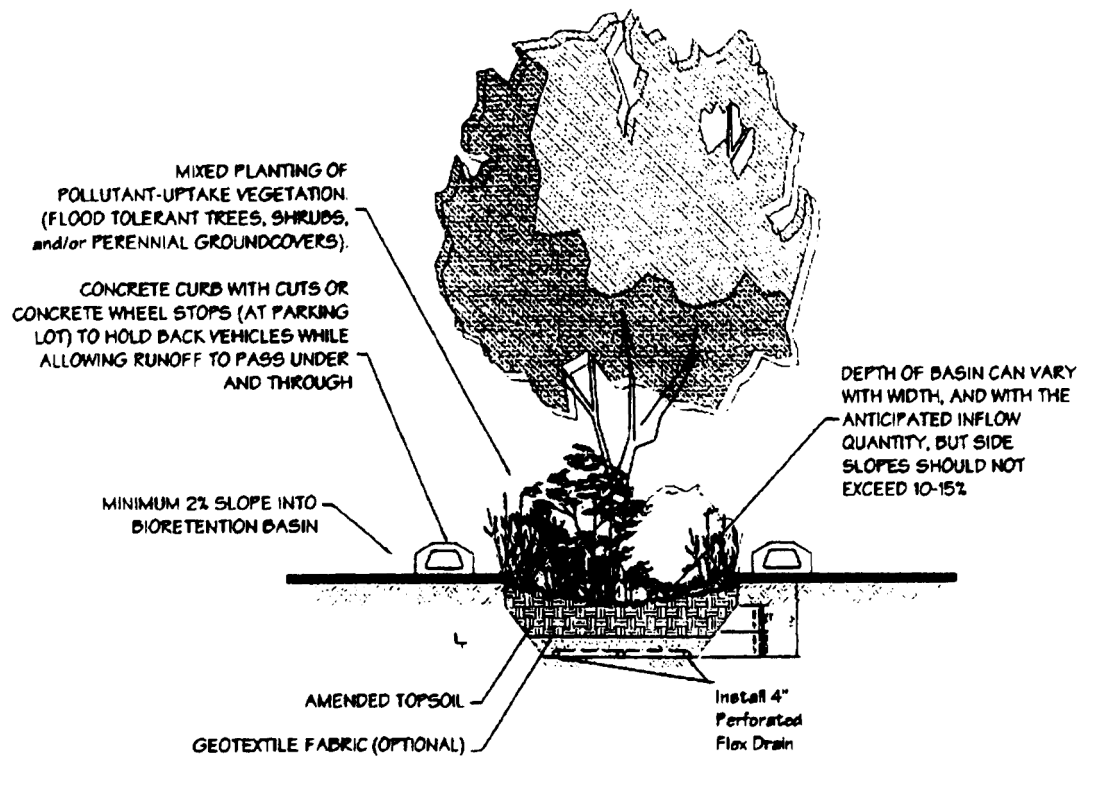
Figure 1: Parking Island Bioretention Cell Cross Section
