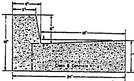
Monolithic Curb & Gutter
