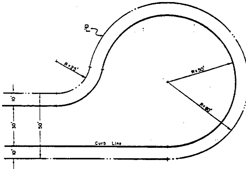
Typical Cul-De-Sac Scale: 1" = 30'
