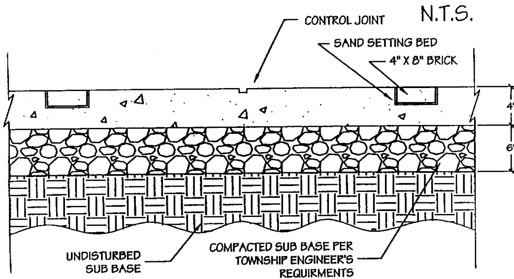
PLAN SECTION
