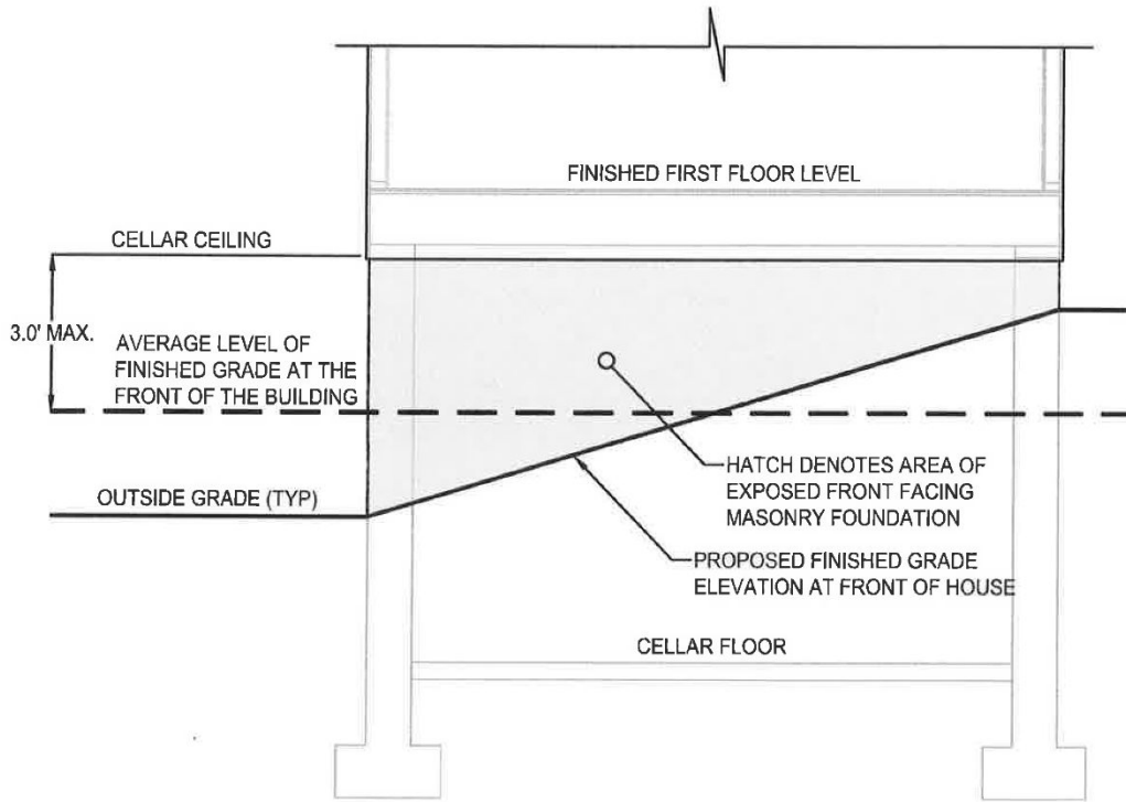
FRONT ELEVATION (SECTION VIEW)
