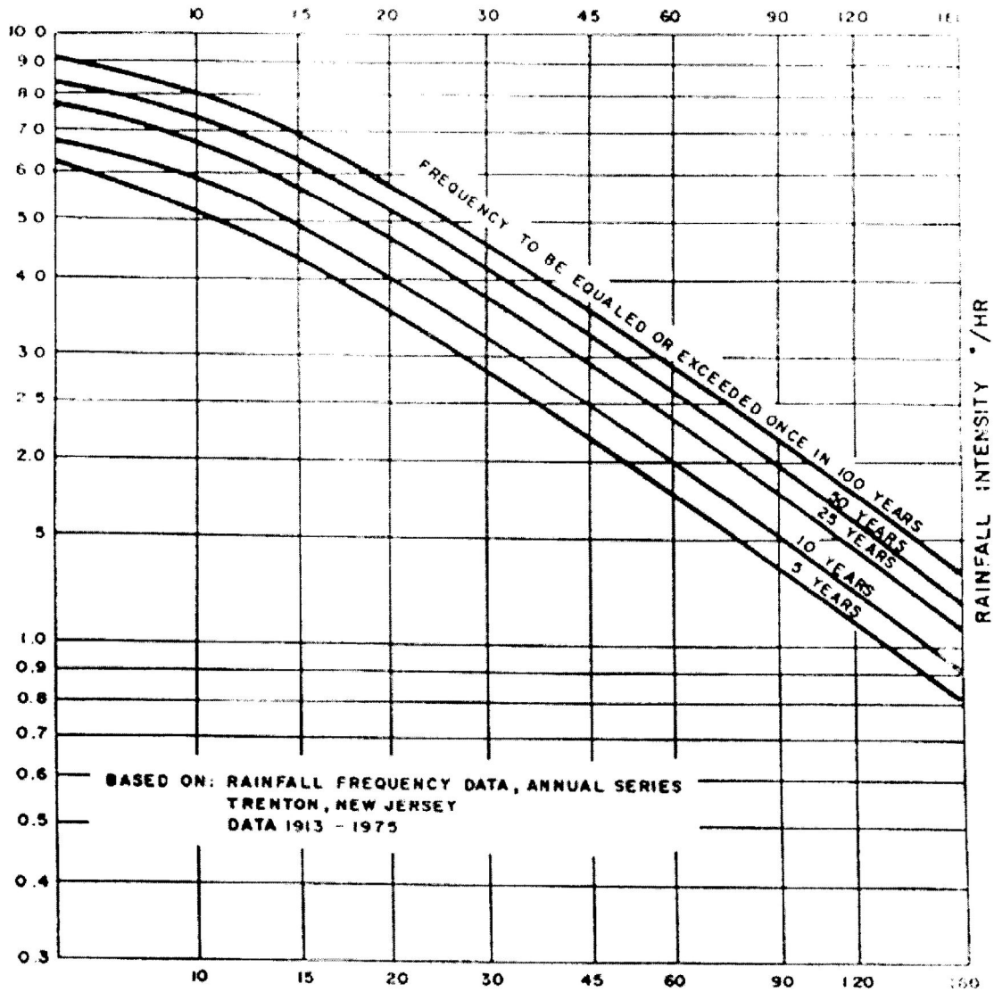
Figure 2: Rainfall Intensity Curves
