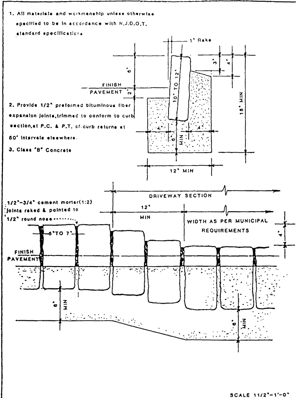
Figure 3A Granite Block Curb
