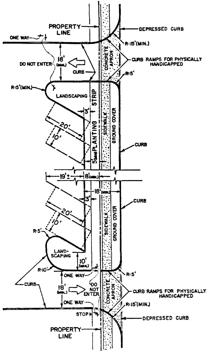
FIGURE 6 ONE WAY ACCESS DRIVES WITH 60° ANGLE PARKING STALLS ABUTTING SAFETY ISLAND (Scale: one inch equals 20 feet)
