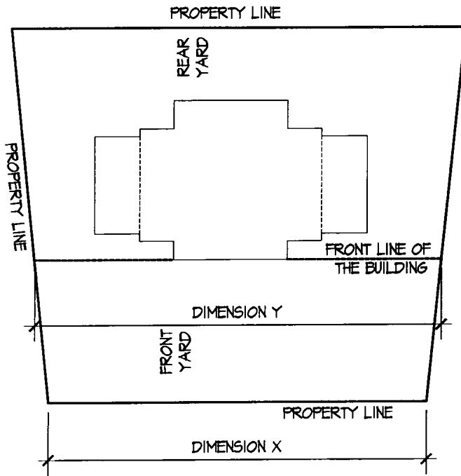
Diagram 4 Irregular Lot Driveway Exhibit
