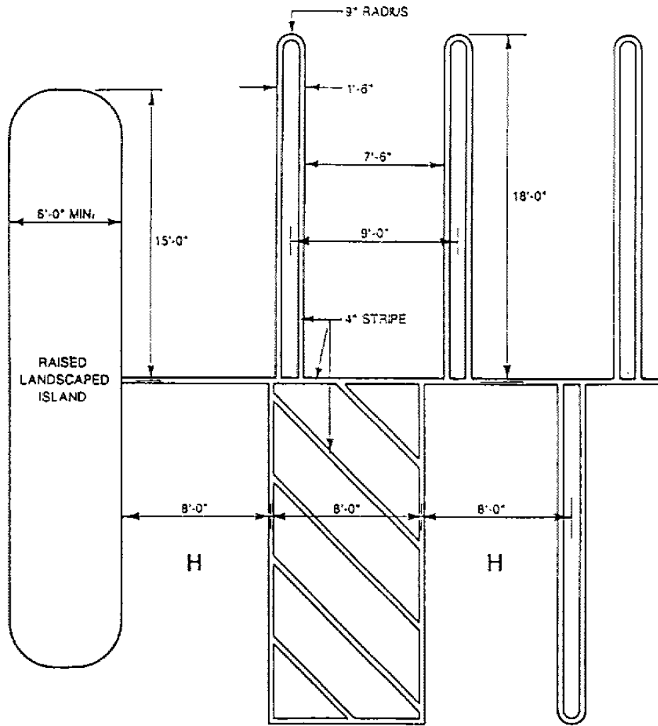
Detail 1: TYPICAL PARKING SPACE DETAILS
