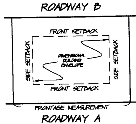
DUAL ACCESS LOT Figure 5.
