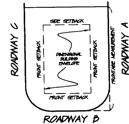
DUAL CORNER LOT Figure 2.
