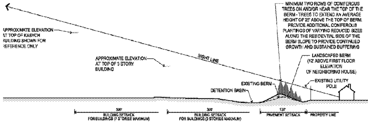
BERM AND BUFFER ALONG EXISTING WEST DETENTION BASIN (TYPICAL) EXHIBIT 1006.4.A.3
