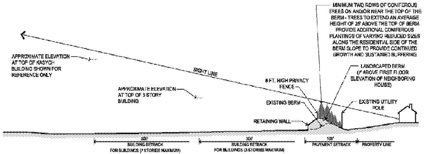
BERM AND BUFFER ALONG RESIDENTIAL PROPERTIES ON SUNSET AVENUE (TYPICAL) EXHIBIT 1006.4.A.4
