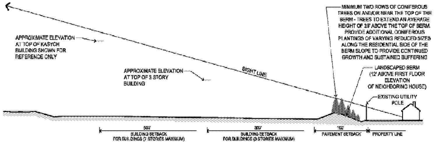
BERM AND BUFFER ALONG RESIDENTIAL PROPERTIES ON PLEASANT AVENUE (EXCLUDING AT DETENTION BASIN) (TYPICAL) EXHIBIT 1006.4.A.2
