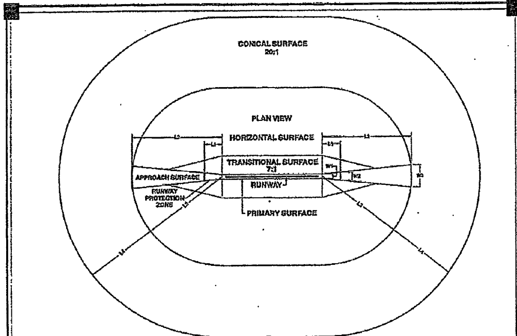
Figure 1: Part 77 Surface Areas
