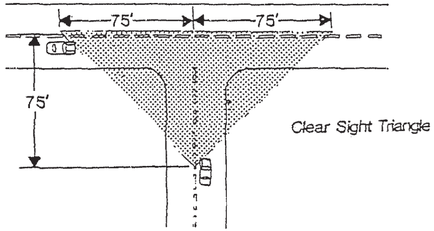
Diagram 3 - CLEAR SIGHT TRIANGLE
