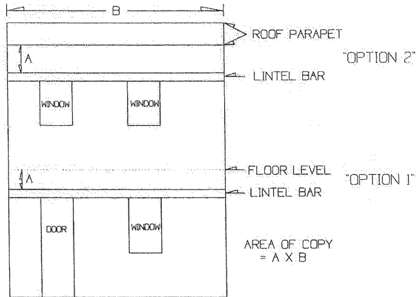
SIGNABLE WALL AREA MULTI-STORY BUILDING
