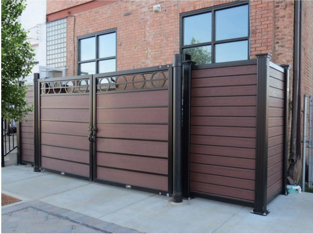
Figure 22: Examples of Dumpster Enclosures
