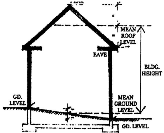
Figure 7: Building Height
