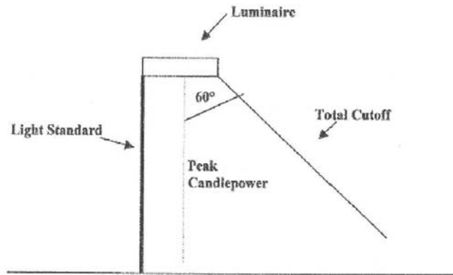
CUTOFF LUMINAIRE
