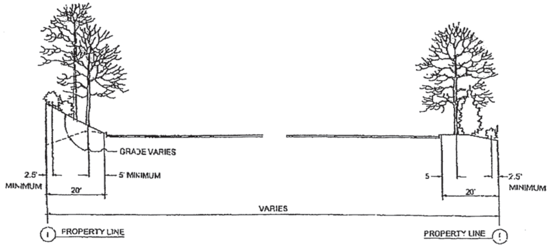
BUFFERYARD '2' CONCEPTUAL SECTION TWENTY FEET WIDE
