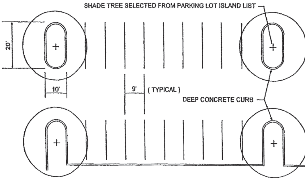
CONCEPTUAL PARKING LOT ISLAND PLANTER PLAN FOR ISLANDS 10' W X 20' L
