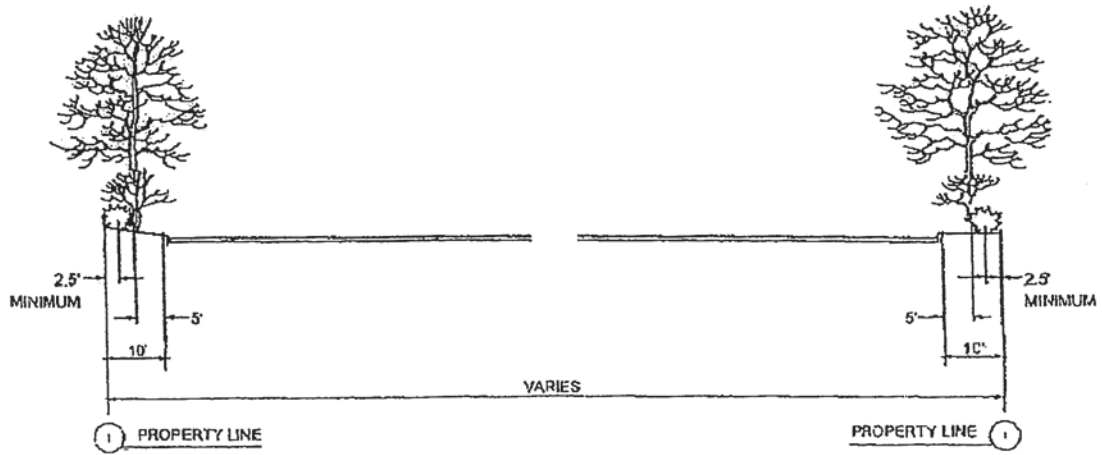
BUFFERYARD '3' CONCEPTUAL SECTION TEN FEET WIDE
