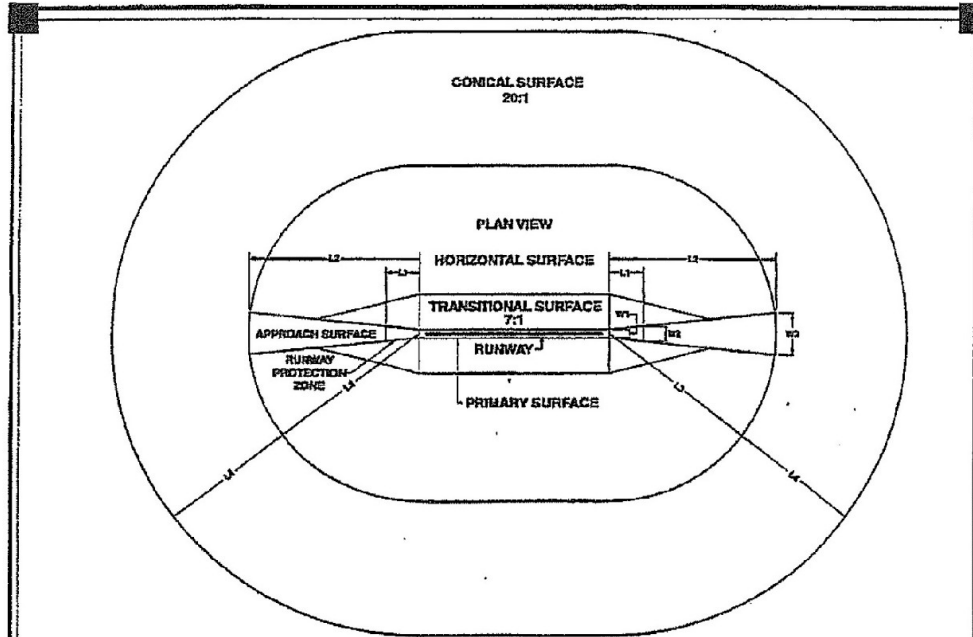
FAR PART 77 "IMAGINARY SURFACES" DIMENSION REQUIREMENTS
