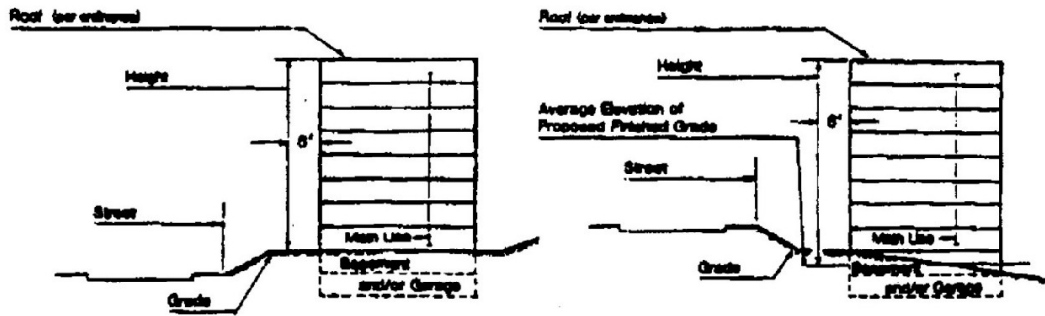
Figure 4: Building Height Measurement
