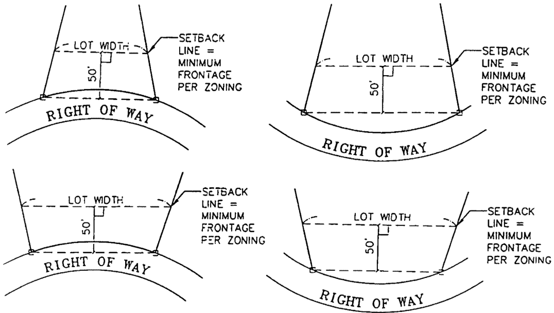
LOT WIDTH DETAIL NOT TO SCALE
