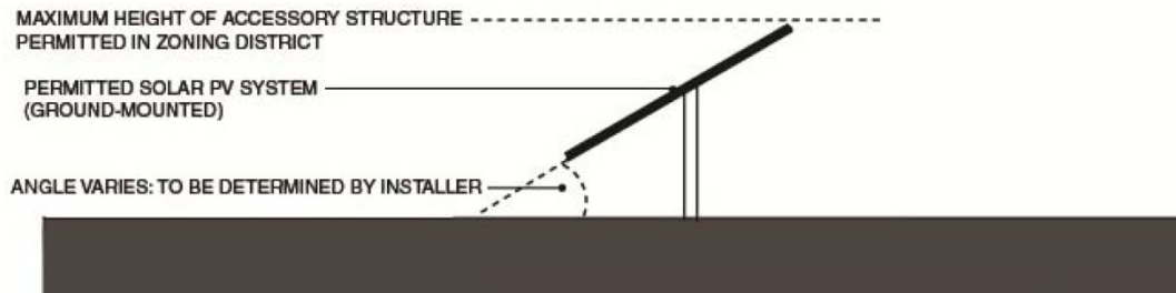
Graphic 5: Height Restriction: Ground-Mounted Solar PV System Elevation
